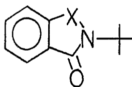
XLVII, X=O LXXXVIIIa, X={C=O} b, X={N-H}
