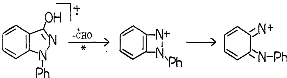
Scheme 26
