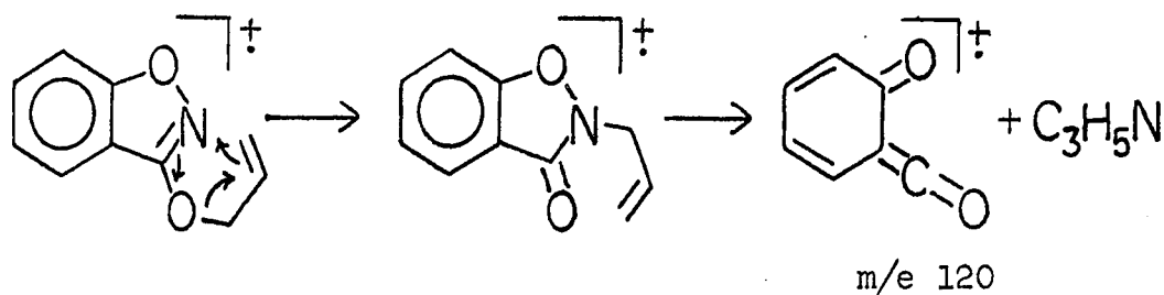
Scheme 13
