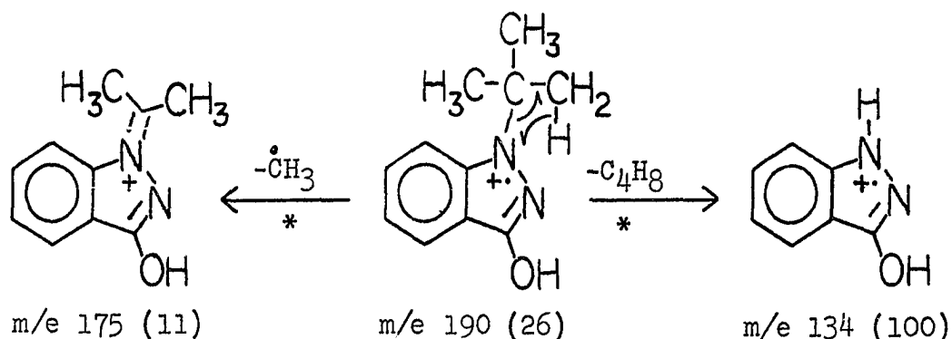
Scheme 27
